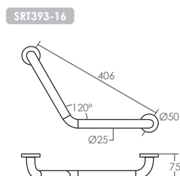
SRT393-16 RM 115 L406xW75mm SRT393-18 RM 119 L457xW75mm Diameter : 25mm
