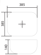
SRTWB1421-RG Dimension : L385xW385xH140mm Rose Gold
