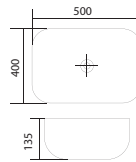
SRTWB1411-RG Dimension : L500xW400xH135mm Rose Gold
