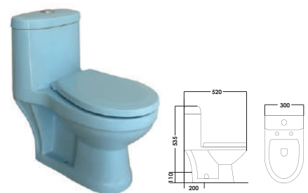
SRTWC203 (BABY WC)
