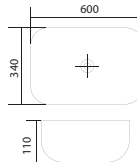
SRTWB1419-GY Dimension : L600xW340xH110mm Golden Yellow
