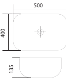
SRTWB1411-GY Dimension : L500xW400xH135mm Golden Yellow
