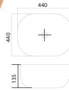
SRTWB1413-RG Dimension : L440xW440xH135mm Rose Gold
