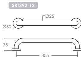
SRT392-12 RM 92 L305xW75xH50mm SRT392-18 RM 106 L457xW75xH50mm SRT392-24 RM 119 L610xW75xH50mm Diameter : 25mm
