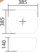
SRTWB1421-RW Dimension : L385xW385xH140mm Rose Gold + White
