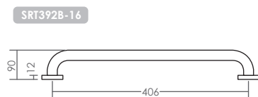
SRT392B-16 RM 158 L406xW90xH80mm Diameter : 32mm
