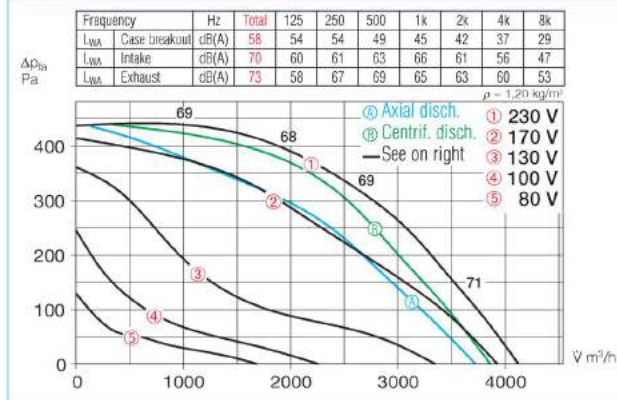
GBW 400/4 T120
