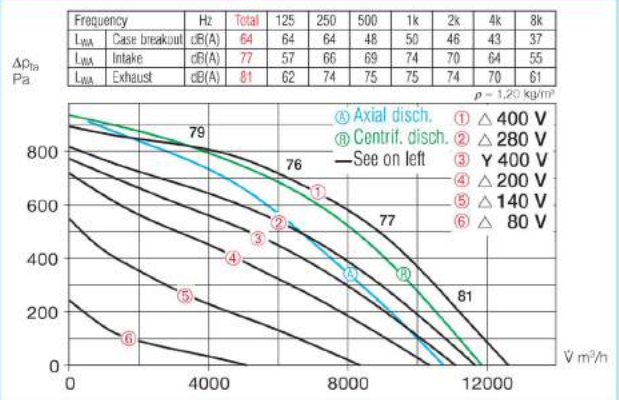
GBW 560/4
